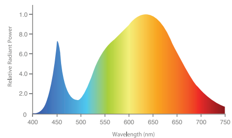
FIG. 5 - Spectral Power Distribution
