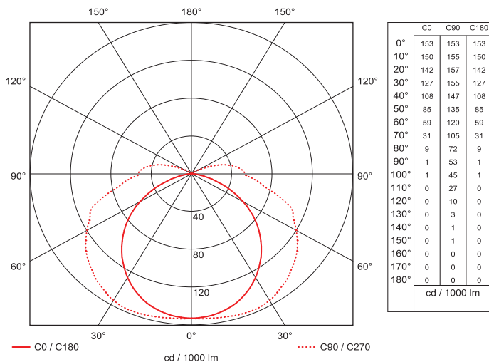
FIG. 1 - Luminance Distribution Chart
