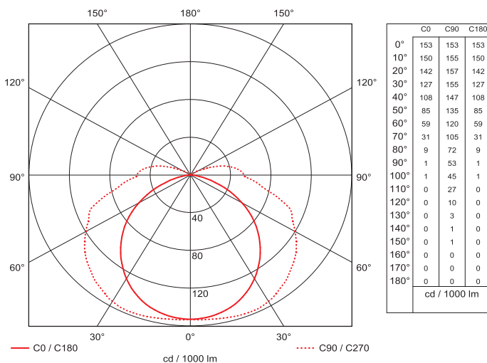
FIG. 1 - Luminance Distribution Chart
