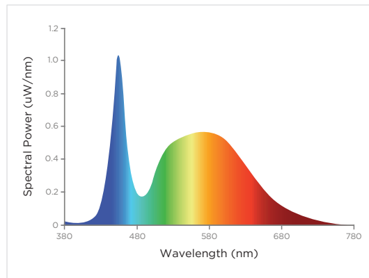
FIG. 4 - Spectral Power Distribution
